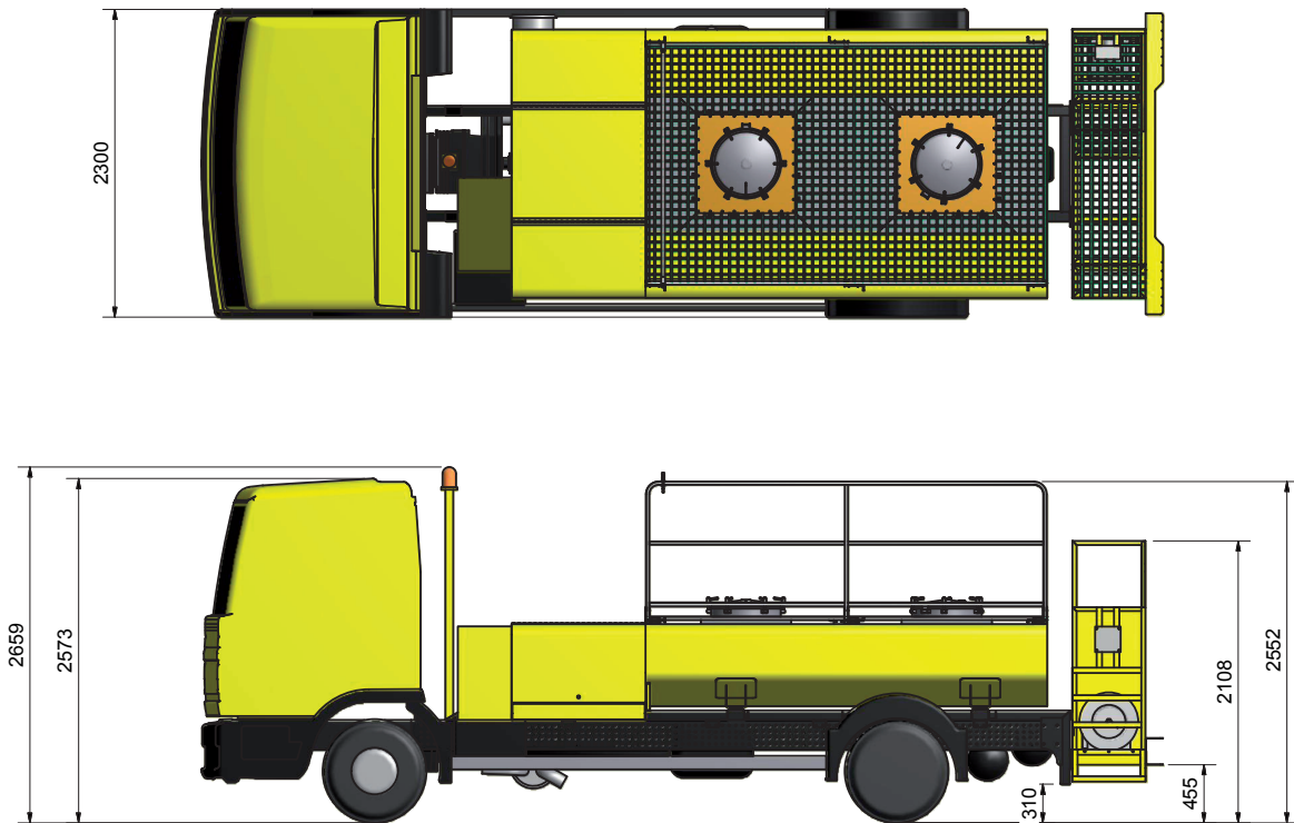
Truck shown in fully laden position
